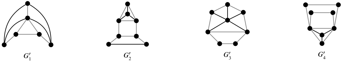
Figure 4: The graphs G'_1 , G'_2 , G'_3 , and G'_4 are matching covered graphs whose perfect matching polytope is box-TDI, yet their matching polytope is not.
