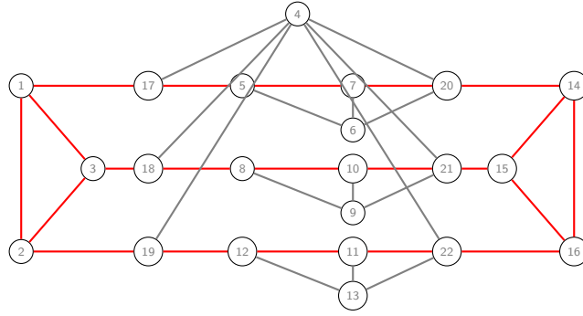
Figure 7: A matching covered graph containing a fully odd subdivision of \overline{C}_6 (in red) as a subgraph and whose perfect matching polytope is box-TDI.
