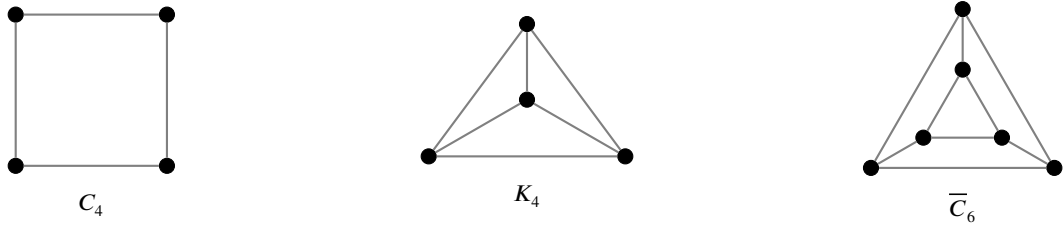
Figure 1: From left to right: the brace C_4 , which is the smallest solid bipartite graph; the brick K_4 , which is the smallest solid nonbipartite graph; the brick \overline{C}_6 , which is the smallest nonsolid brick.
