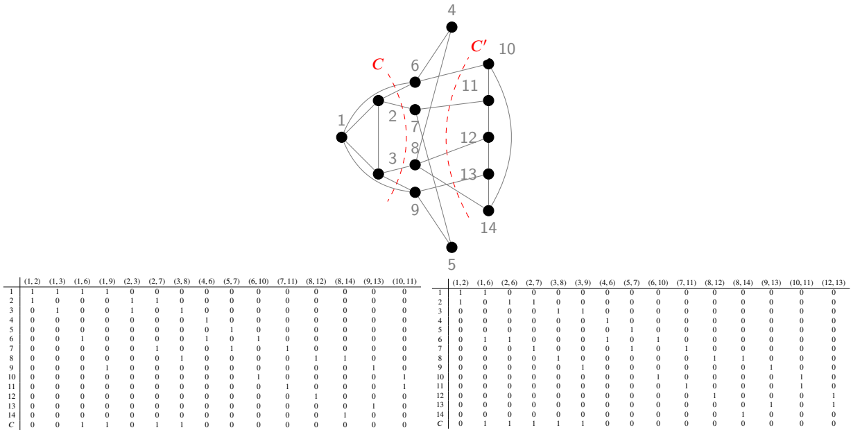
Figure 6: The Moonfish graph \mathcal{M} and the unique maximal inclusionwise laminar family \{C, C'\} of \mathcal{M} . One can check that all C -contractions and C' -contractions are odd intercylic near-bricks. Since, \mathcal{M} has two bricks — K_4 and the odd wheel of order 5 — and the two C -contractions are nonbipartite, \{C\} \in \mathfrak{F}_{\mathcal{M}} . In particular, the two matrices above are nonsingular maximal submatrices of on the M_{\mathcal{M}}^{(C)} and have —from left to right— determinant 4 and 8, up to the sign. Then, the matrix M_{\mathcal{M}}^{(C)} is nonequimodular, by definition, and it is face-defining for the affine hull of P(\mathcal{M}) by Theorem 9. By Theorem 11, P(\mathcal{M}) is not box-TDI.
