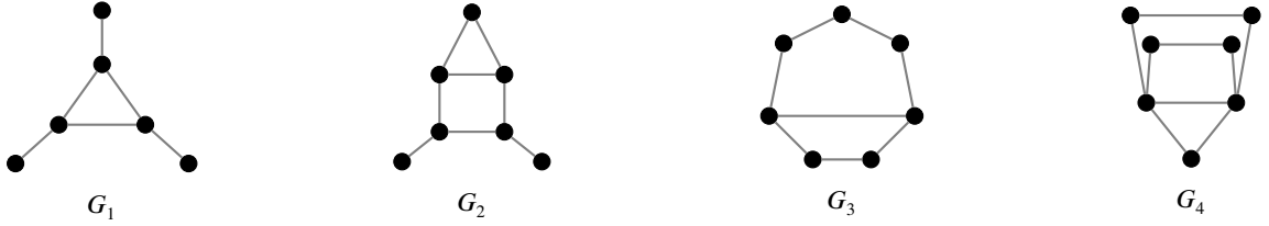
Figure 3: The graphs G_i , i = 1, 2, 3, 4 , are the subgraphs that prevent the matching polytope from being box-TDI (up to fully odd subdivision).
