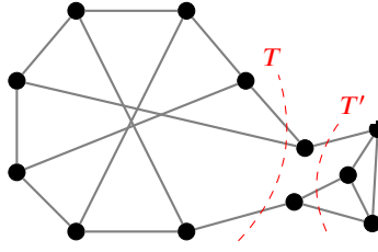
Figure 8: A nonplanar nonbipartite cubic graph with two nontrivial tight cuts T and T' , which is 3-edge-colorable by Corollary 25.
