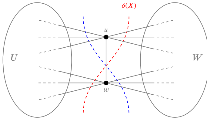
Figure 5: The two 2-separation cuts with respect to u and w are drawn in red and blue. Note that u and w may be nonadjacent.
