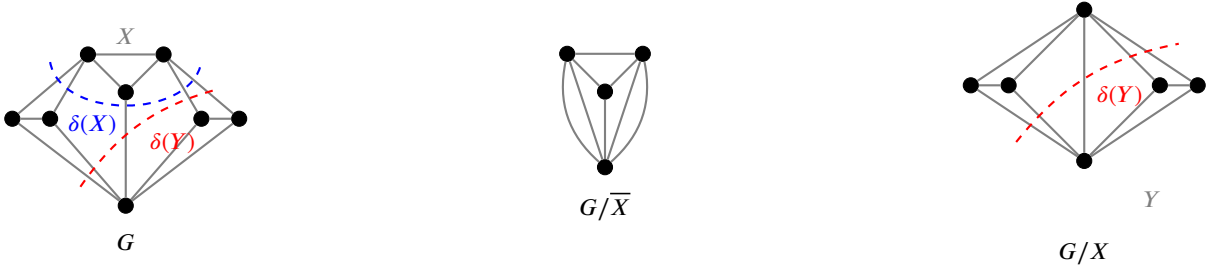
Figure 2: A matching covered graph G , and a maximal inclusionwise laminar family of tight cuts \mathcal{F} = \{\delta(X), \delta(Y)\} . As \mathcal{F} \in \mathfrak{F}_G , G has three bricks. In particular, one can see the two \delta(X) -contractions G/X and G/\bar{X} . While G/\bar{X} is already one of the bricks of G , G/X still has two bricks that one can identify by computing G/X/Y and G/X/\bar{Y} . All of these bricks are isomorphic to K_4 , up to parallel edges.
